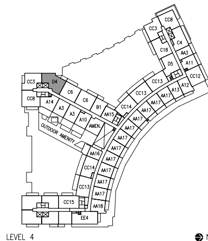
LEVEL 4 NORTH
