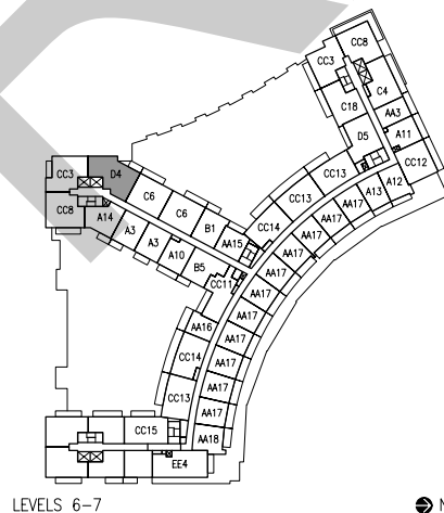
LEVELS 6-7 NORTH
